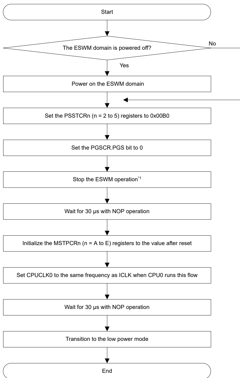
Figure 11.11 Additional flow for the transition to Software Standby mode and Deep Software Standby mode 1/2/3
